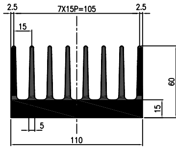
F60110R 8.10Kg/m
