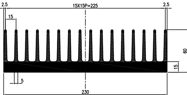
F60230R 16.65Kg/m
